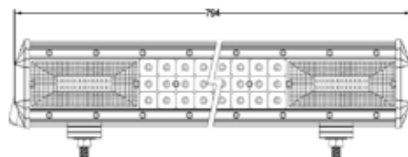
432 WATTS 144 LEDS X 3 WATTS LW-FKM-432W PZA
