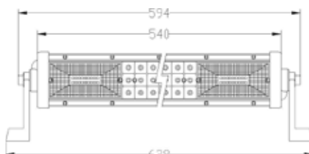
270 WATTS 90 LEDS X 3 WATTS LW-GKN-270W PZA
