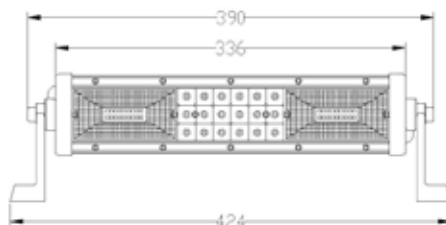
162 WATTS 54 LEDS X 3 WATTS LW-GKN-162W PZA
