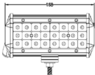
72 WATTS 24 LEDS X 3 WATTS LW-FKM-072W PZA
