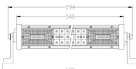
678 WATTS 225 LEDS X 3 WATTS LW-GKN-678W PZA
