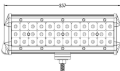
108 WATTS 36 LEDS X 3 WATTS LW-FKM-108W PZA
