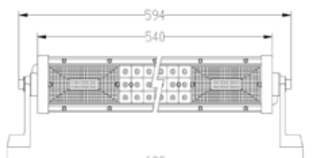
405 WATTS 135 LEDS X 3 WATTS LW-GKN-405W PZA
