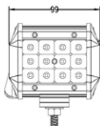
36 WATTS 12 LEDS X 3 WATTS LW-FKM-036W PZA
